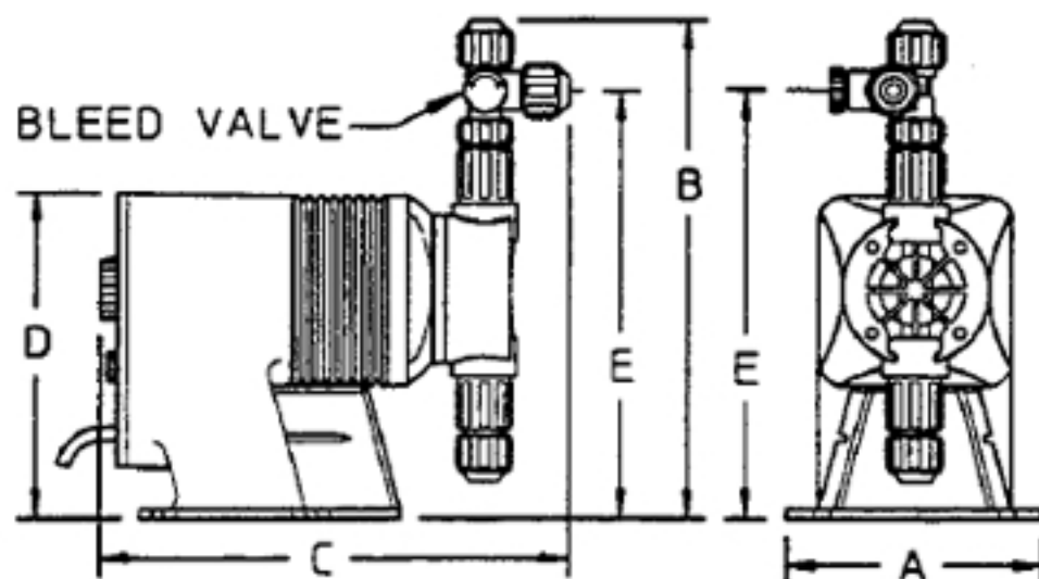
Series A PLUS Dimensions (inches)
