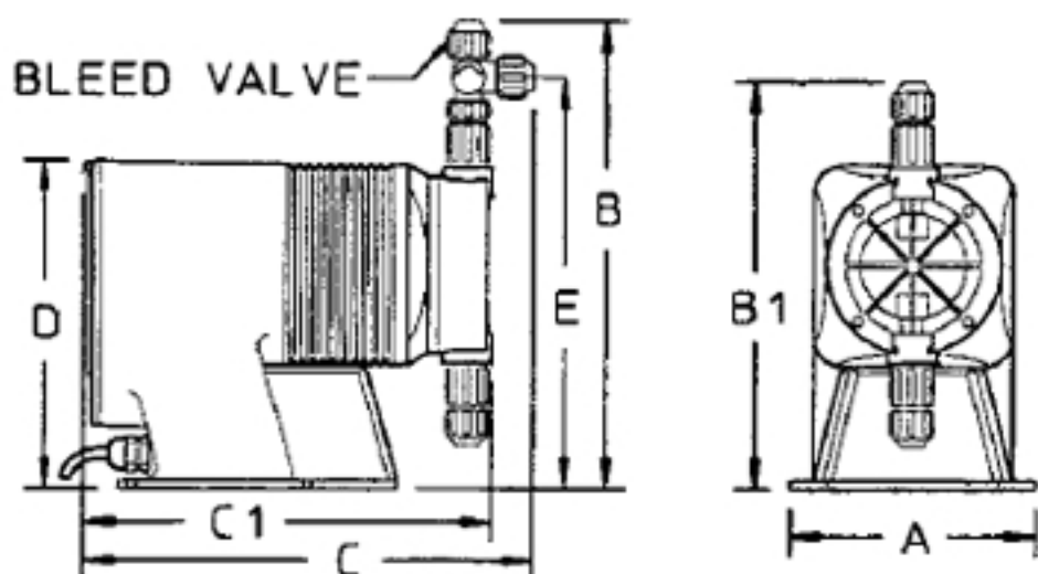
Series ET Dimensions (inches)
